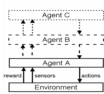
Fig. 1: Connection between agent and environment. Inner mechanisms of the agent could be seen as environment for another (copy of the) agent - this is the way how to easily create sophisticated control hierarchy.
