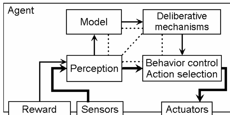
Fig. 2: Intelligent agent architecture.
