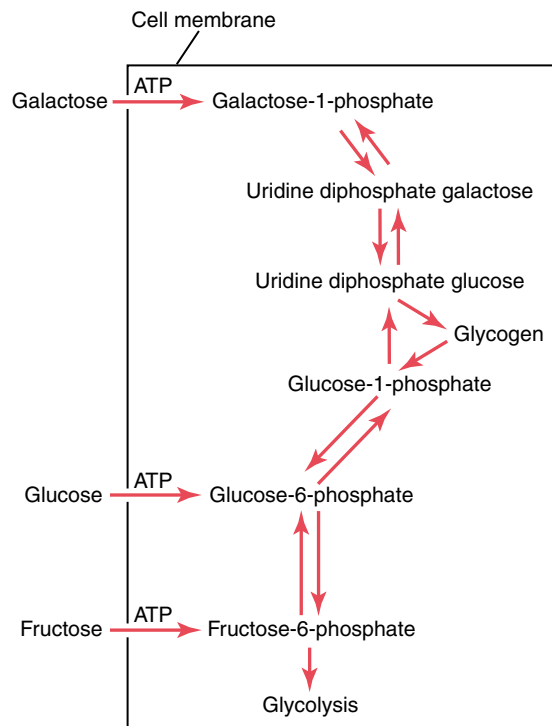
Figure 67-3 Interconversions of the three major monosaccharides—glucose, fructose, and galactose—in liver cells.
