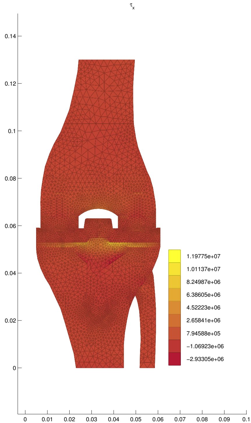
Figure 23: Stresses \tau_x
