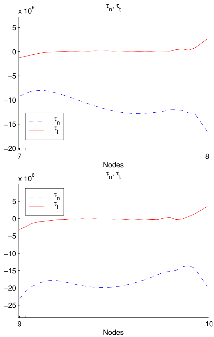
Figure 28: A normal and tangential components of stress on contact boundary.
