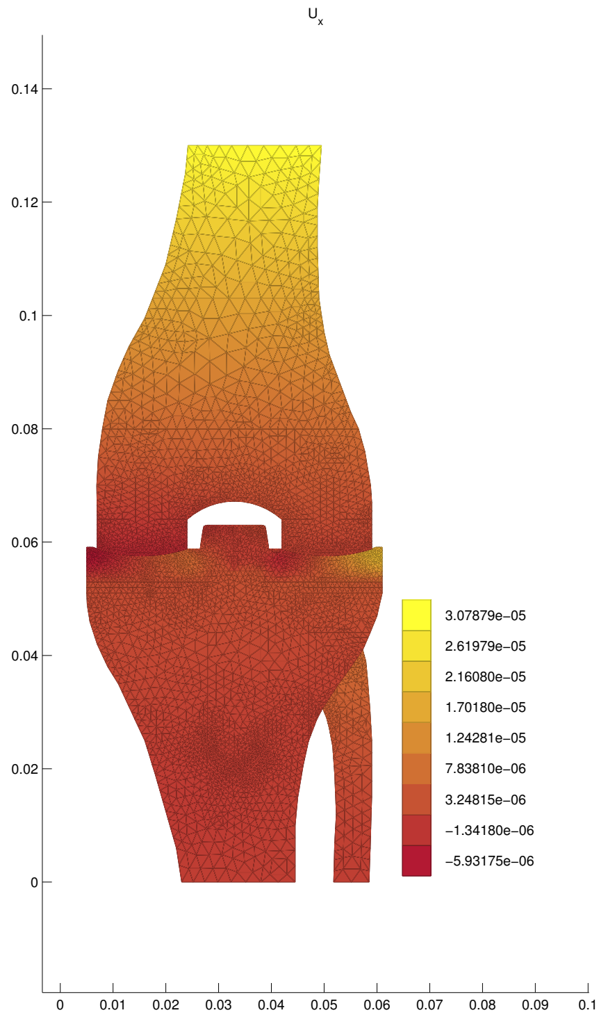
Figure 21: Horizontal component of displacement
