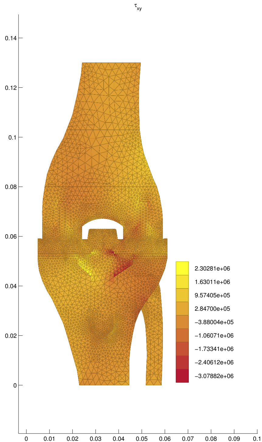
Figure 25: Stresses \tau_{xy}
