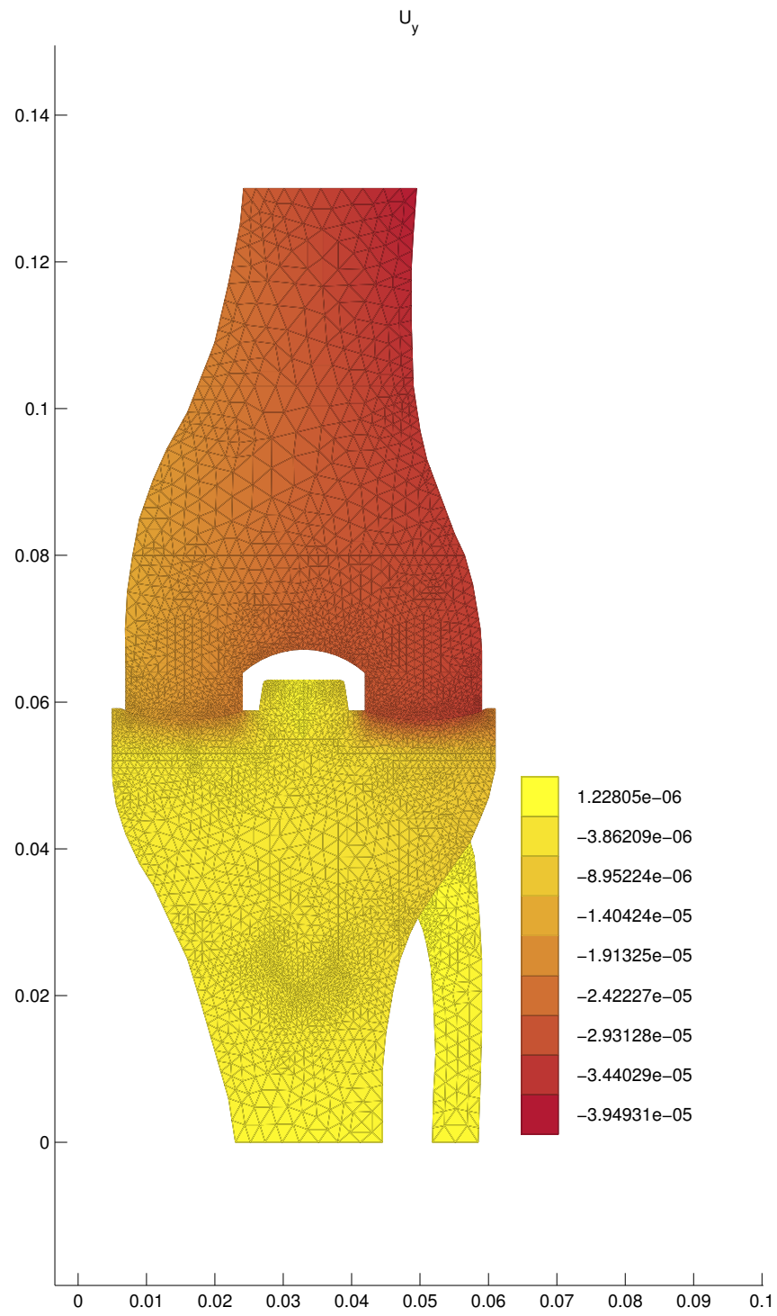
Figure 22: Vertical component of displacement
