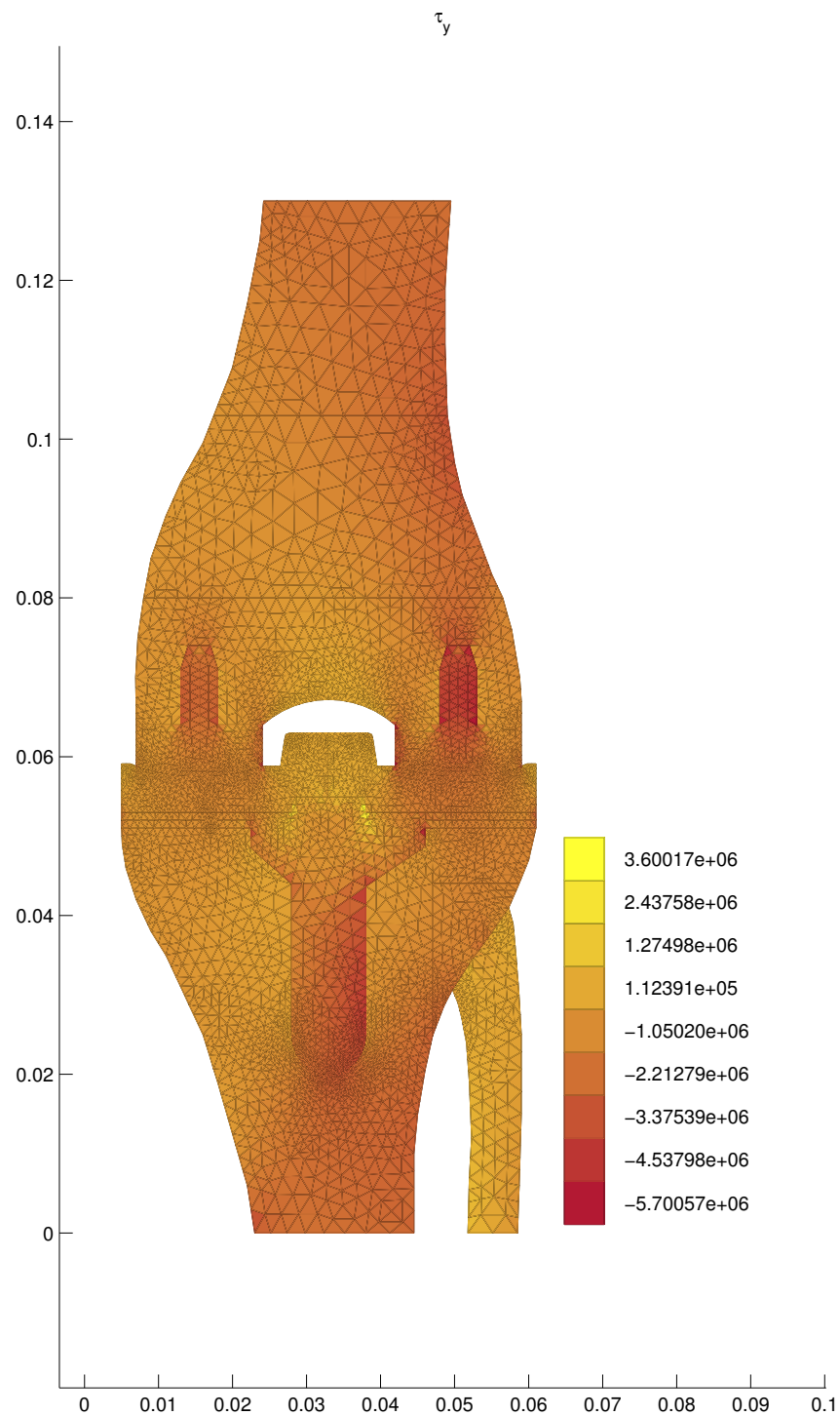
Figure 24: Stresses \tau_y
