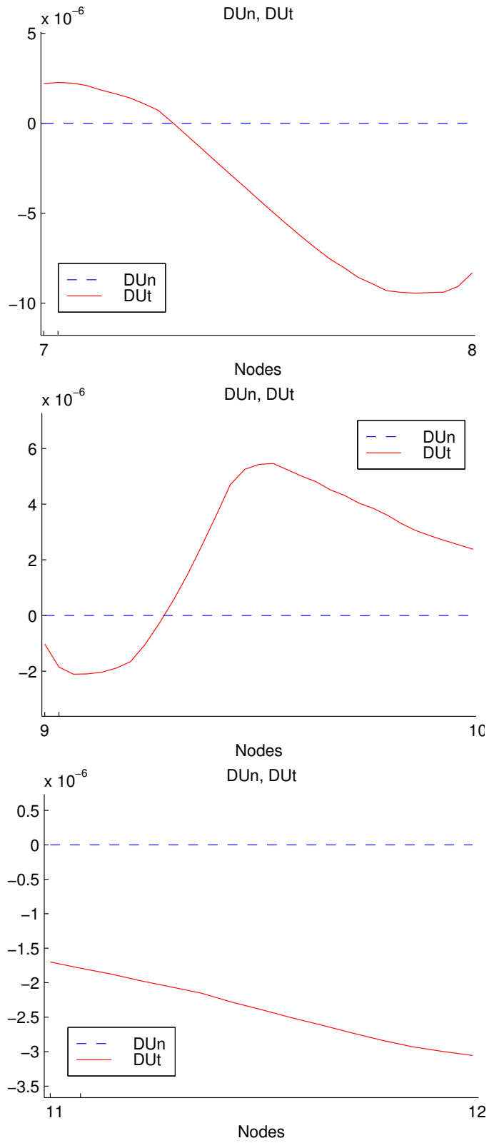
Figure 27: A normal and tangential components of displacement on contact boundary.
