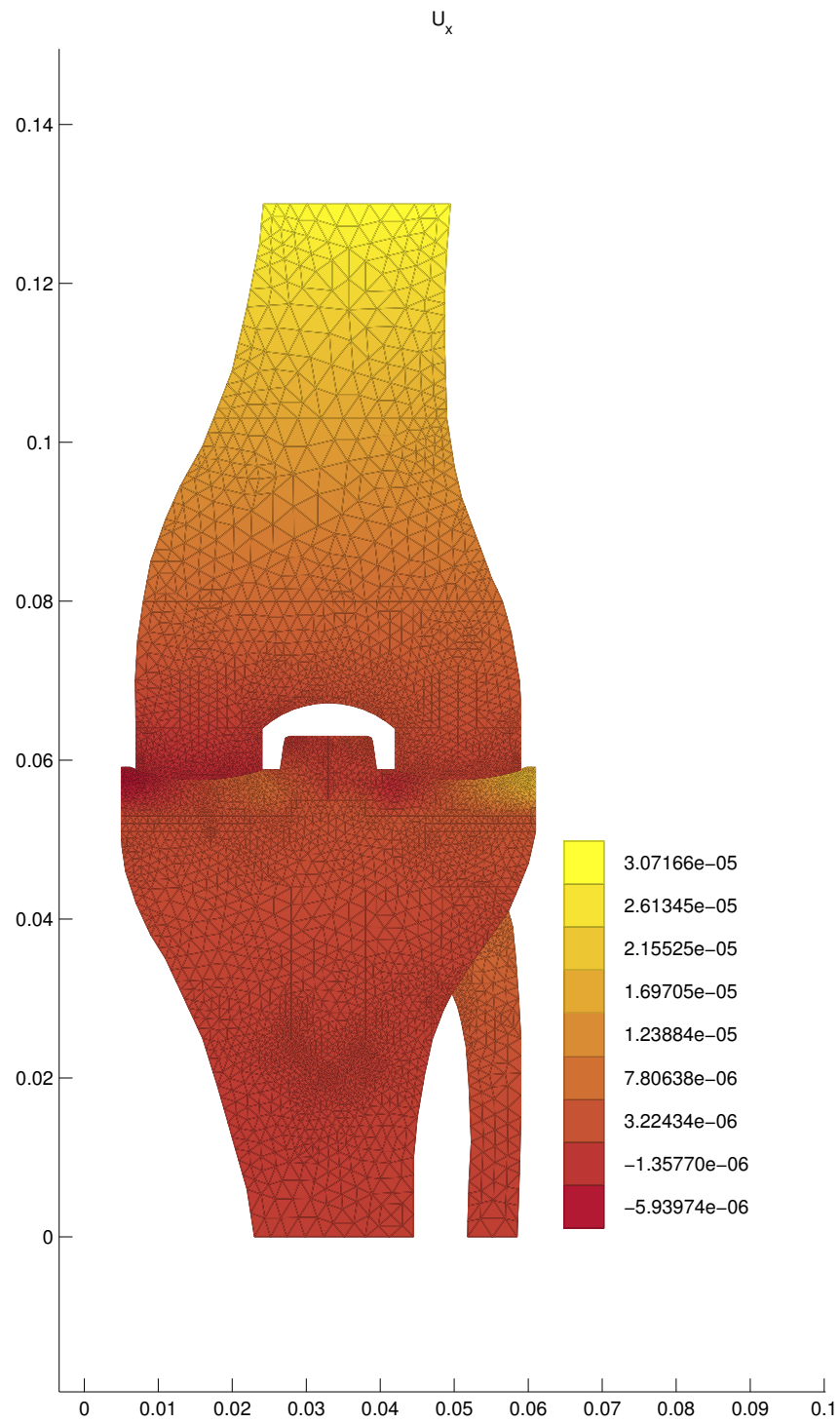
Figure 31: Horizontal component of displacement
