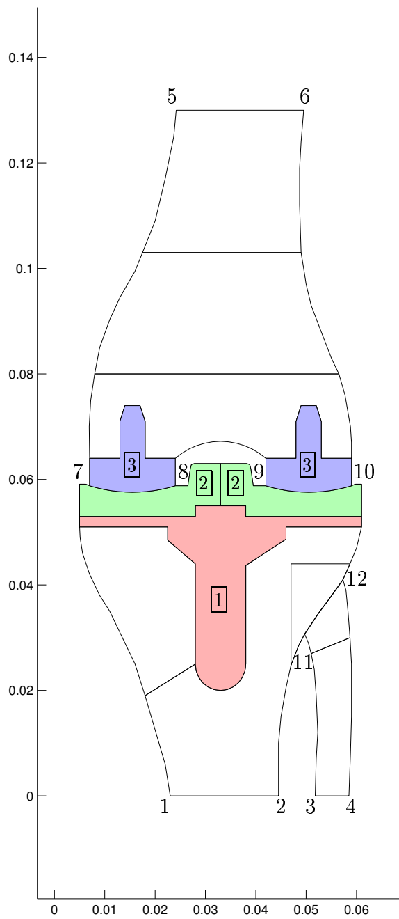
Figure 29: Geometry
