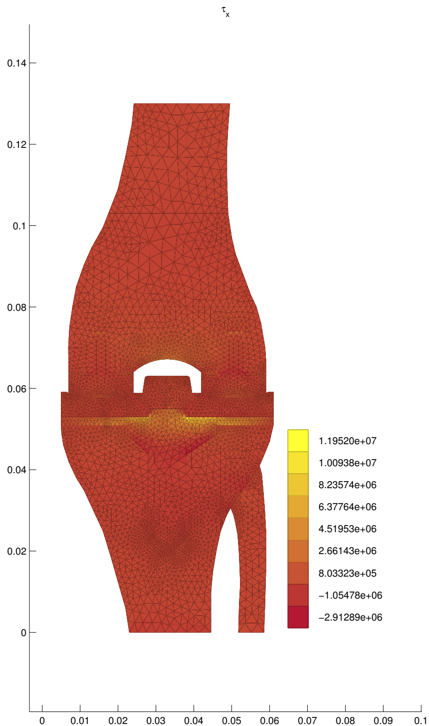
Figure 33: Stresses \tau_x
