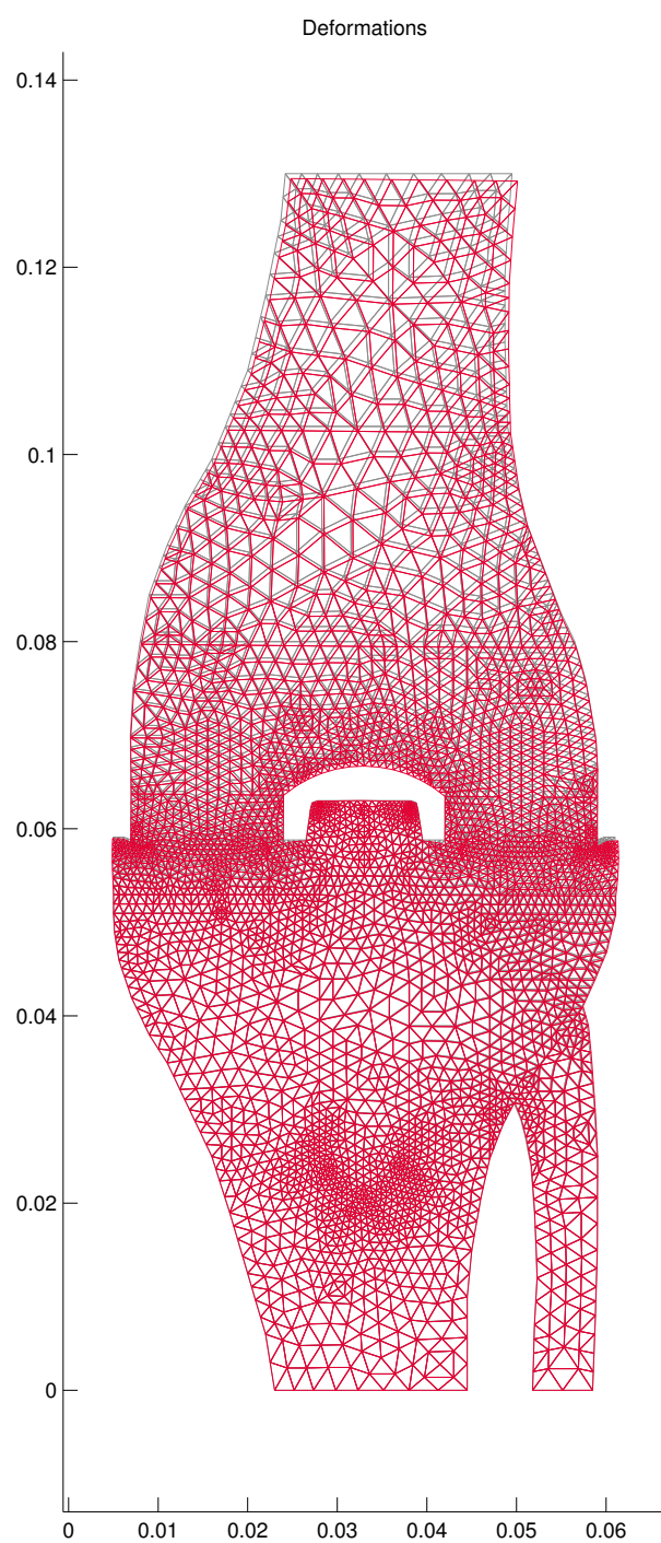
Figure 30: Deformations (enlarge factor=20)
