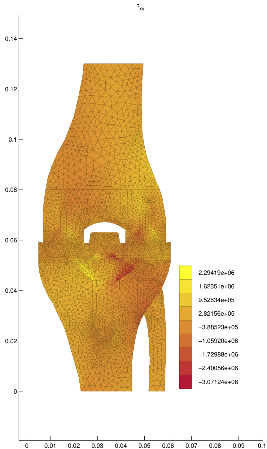
Figure 35: Stresses \tau_{xy}
