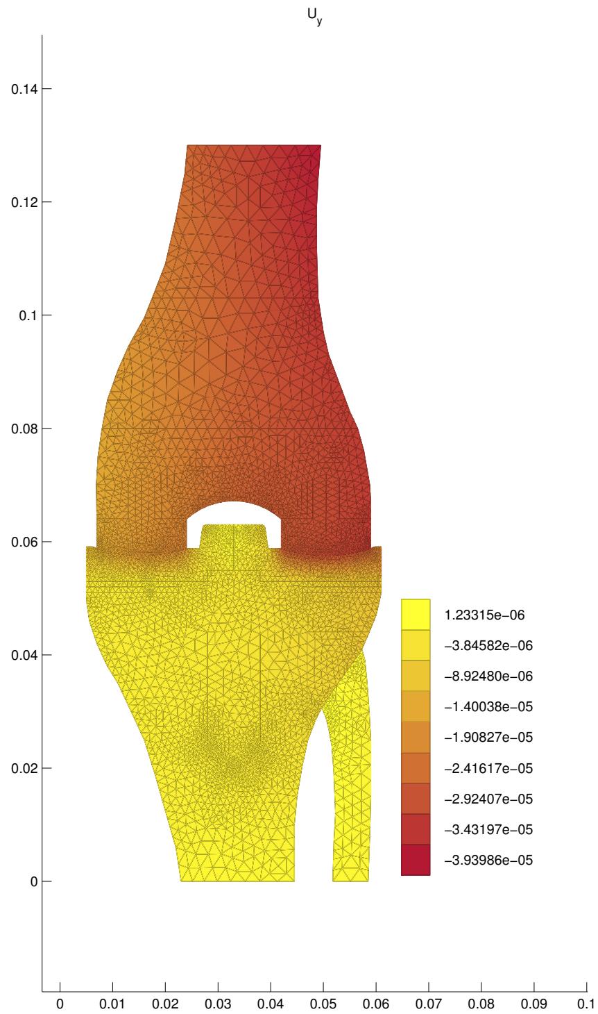
Figure 32: Vertical component of displacement
