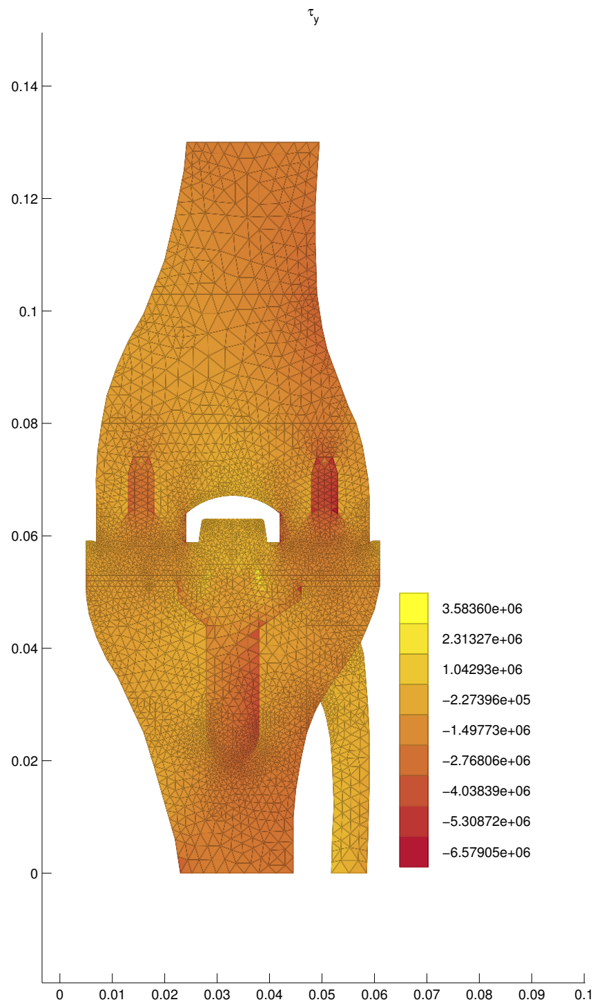
Figure 34: Stresses \tau_y
