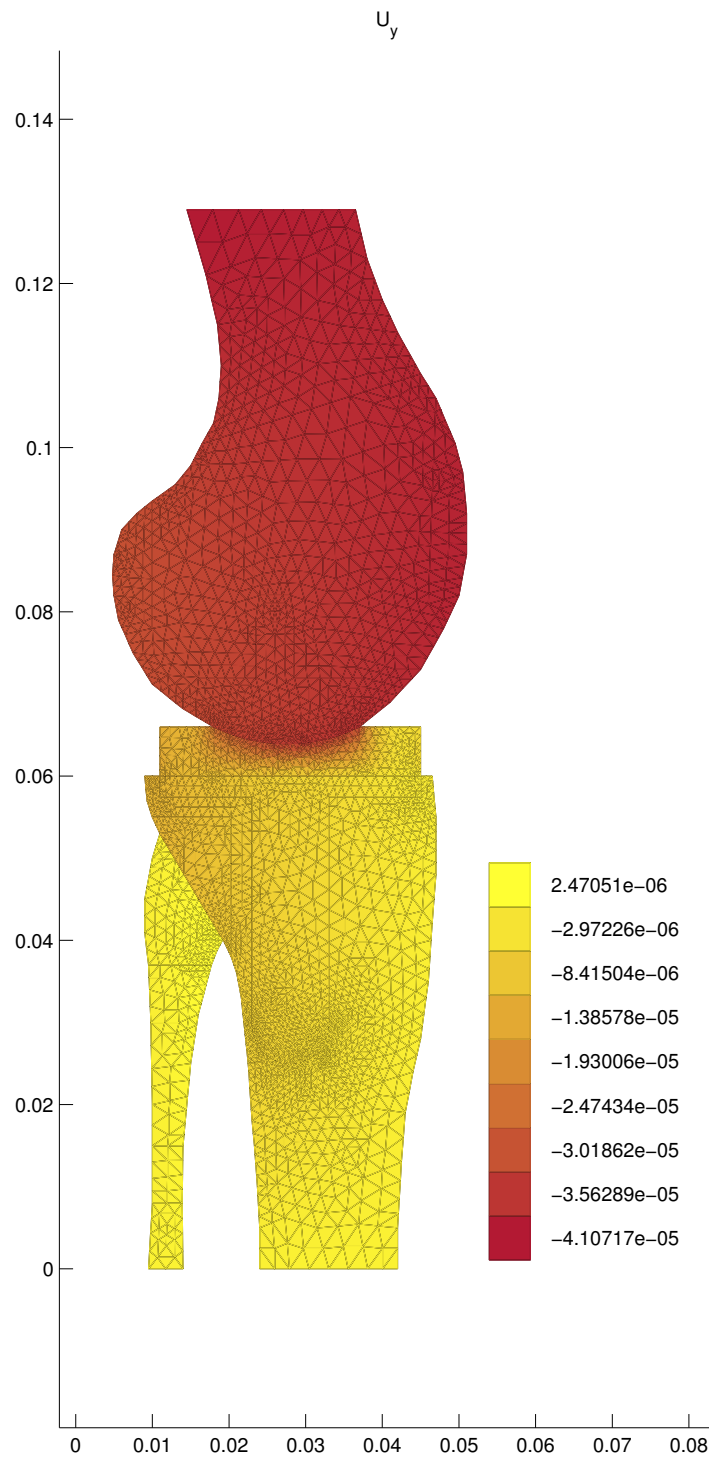
Figure 50: Vertical component of displacement
