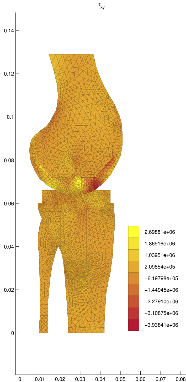
Figure 53: Stresses \tau_{xy}
