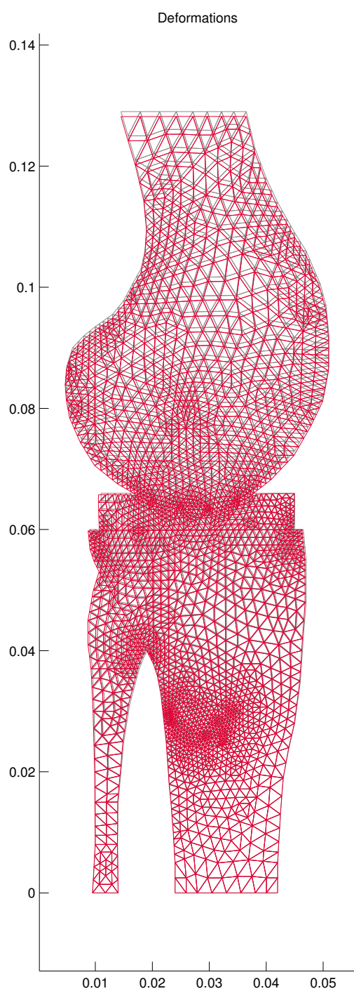
Figure 48: Deformations (enlarge factor=20)
