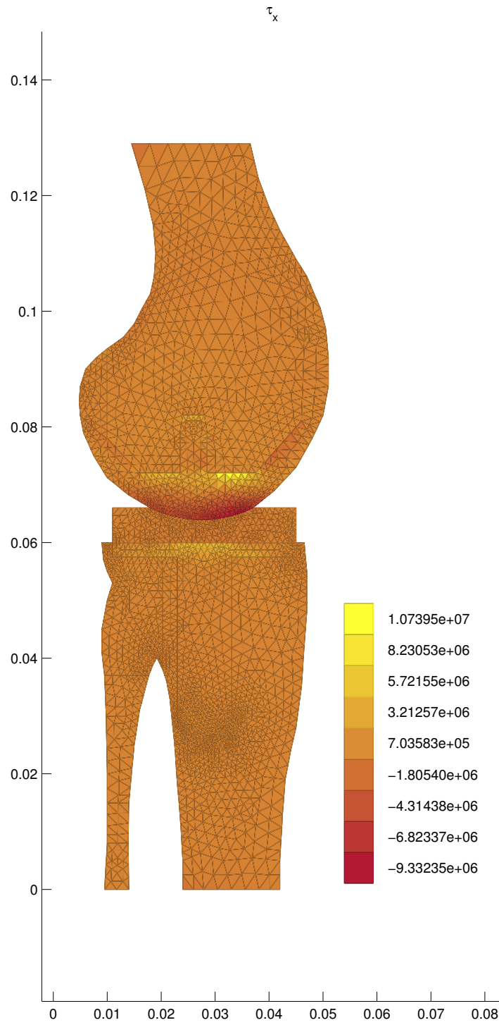
Figure 51: Stresses \tau_x
